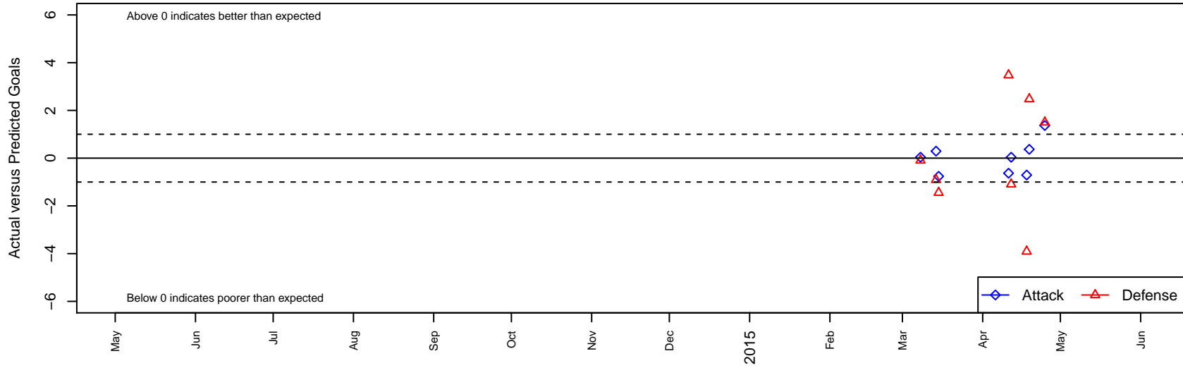
THUSC Redstar Rapids Black G02 Dots are actual minus expected GF (blue circles) and GA (red triangles). Blue line is smoothed change in attack strength. Red is smoothed change in defense strength.
